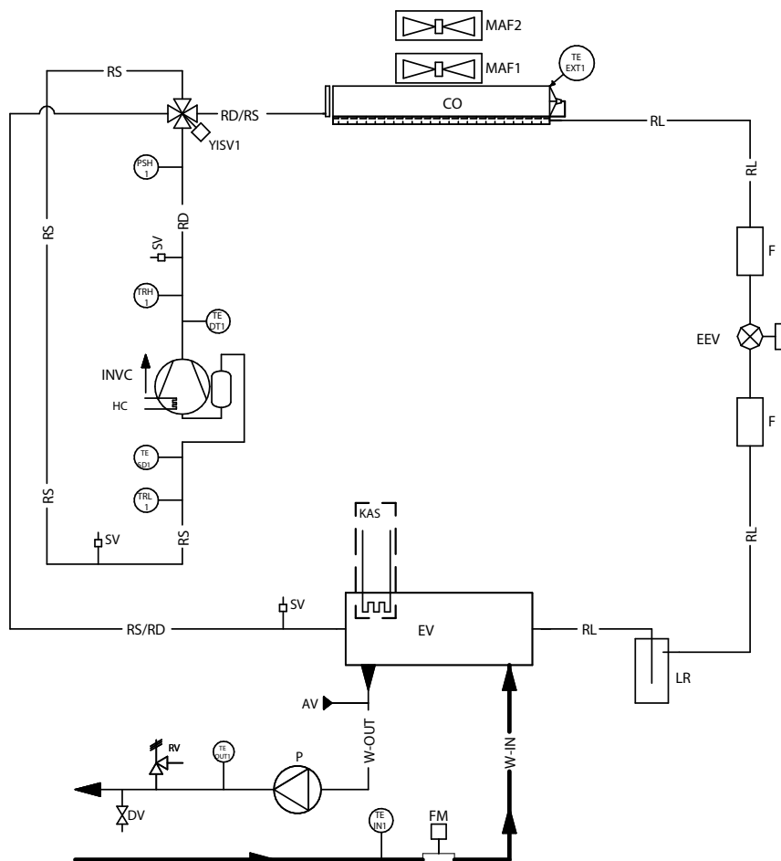
Circuit diagram i-290 0112, 0115, 0118
